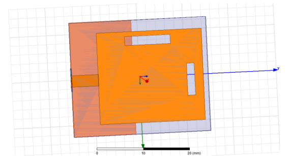
Fig.2 (a): Top view of Proposed Antenna
