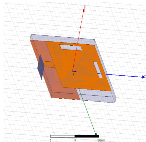
Fig.1: Structure of Proposed Antenna
