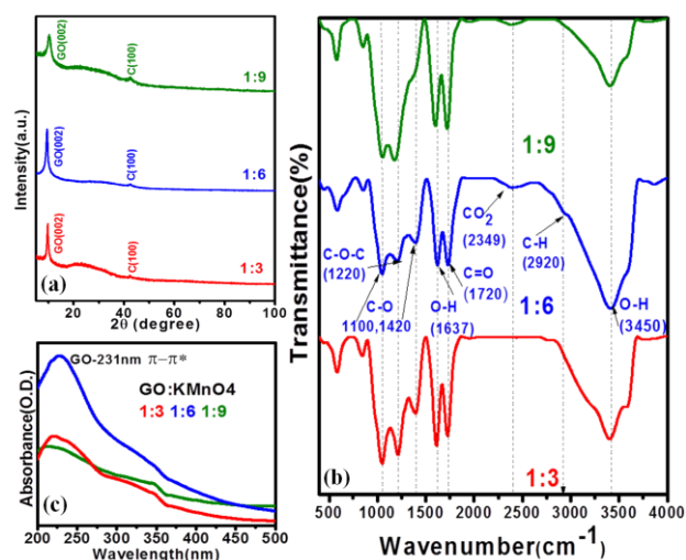
Fig. 2 (a) XRD patterns, (b) FTIR spectra and (c) UV-Vis spectra of different GO samples synthesized for different concentration of oxidizing agent with graphite: \text{KMnO}_4 ratio as 1:3, 1:6 and 1:9 wt.%.
