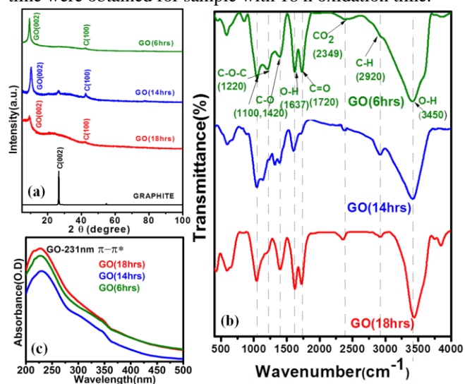
Fig. 1 (a) XRD pattern, (b) FTIR spectra and (c) UV-Vis spectra of different GO samples synthesized for different oxidation time.
