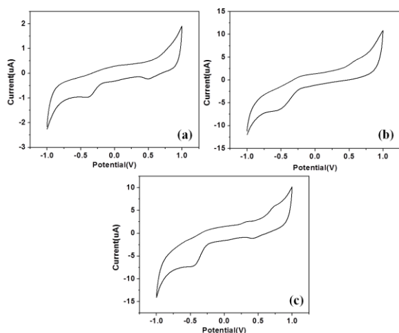
Fig. 3 Cyclic voltammograms of (a) GO, (b) GO/MCF-7 cells and (c) GO/HeLa cells in the potential range -1.0 to 1.0V versus Ag/AgCl at a scan rate of 50 mV/s.
